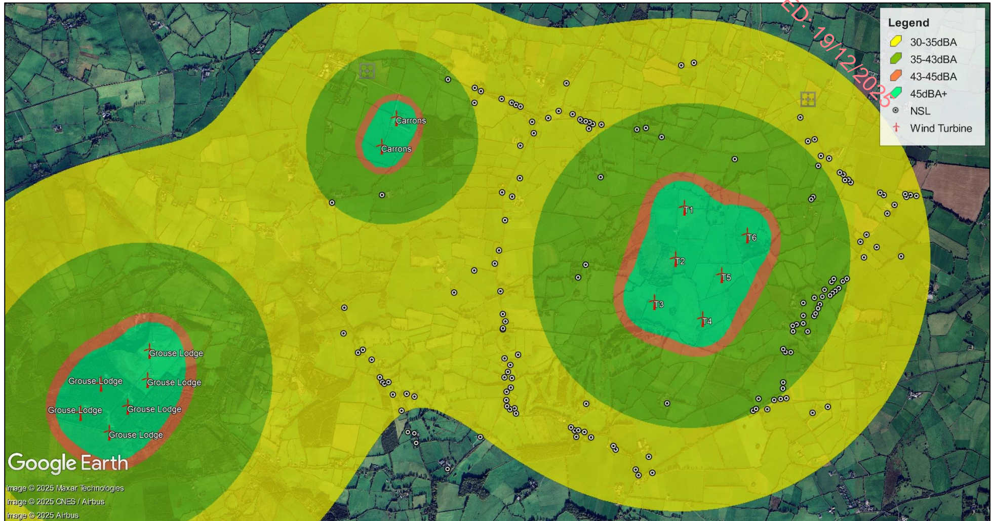
Figure 1: Noise Contours at 4m height
